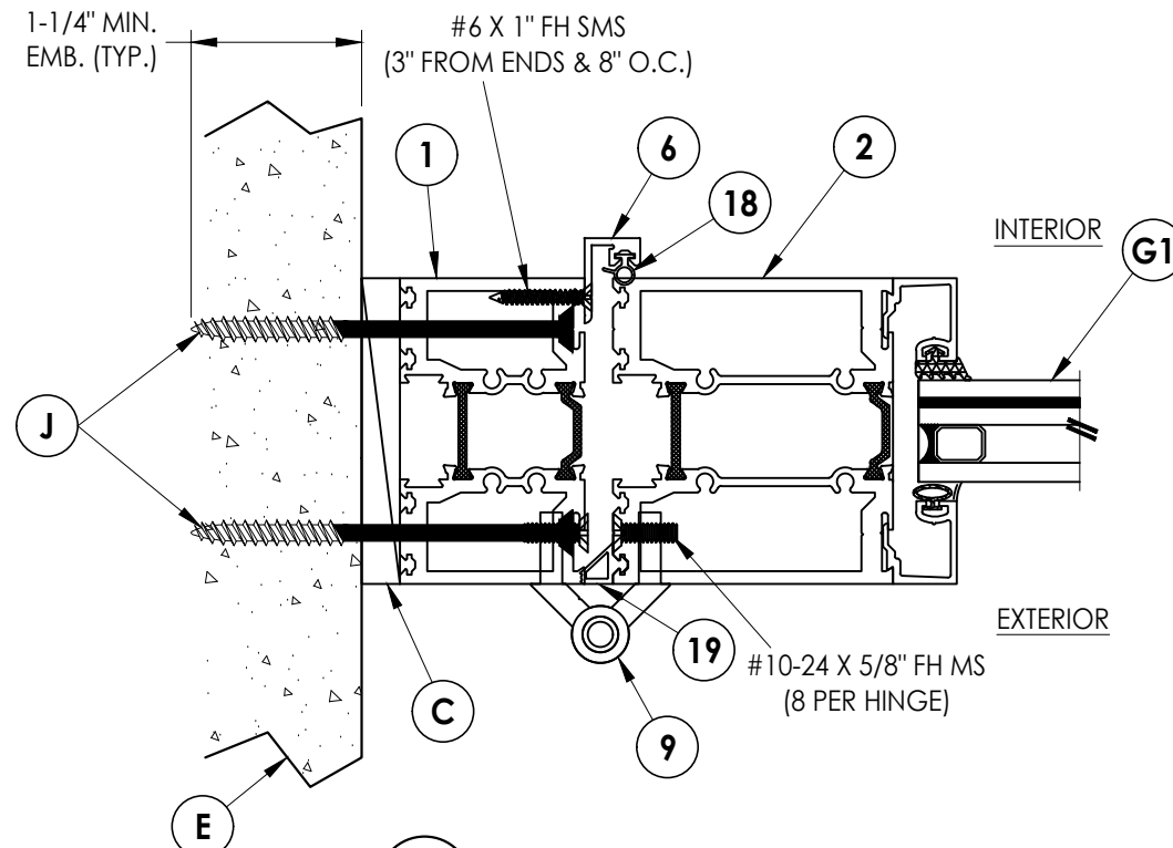
4 7 HORIZONTAL CROSS SECTION Shown Direct to Masonry
