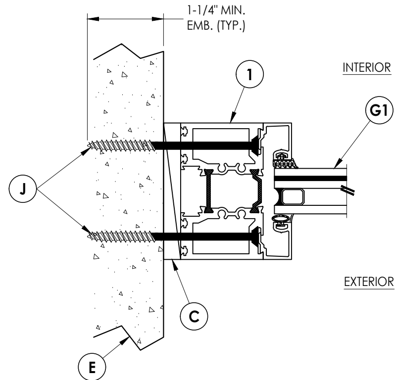
3 7 HORIZONTAL CROSS SECTION Shown Direct to Masonry
